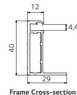
Frame Cross-section
